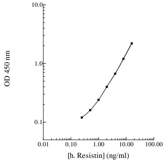
H. Resistin Standard Curve
